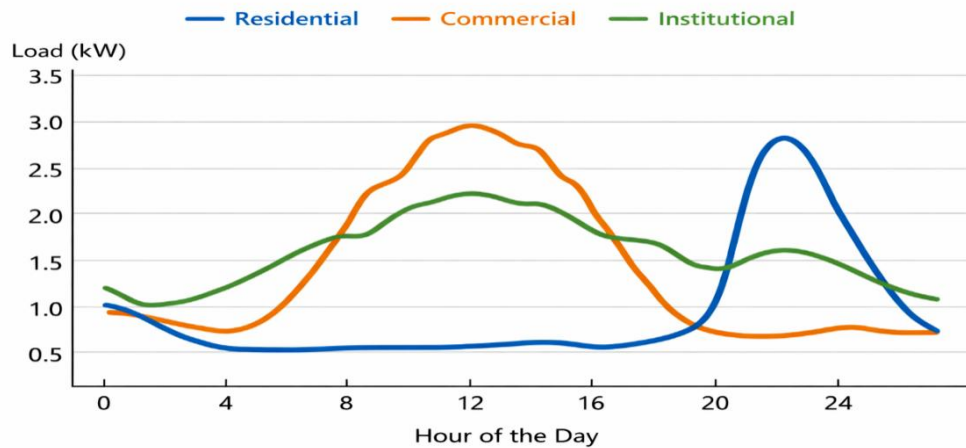
Figure 4.2. Hourly Load Profiles for Three Representative Community Load Archetypes
