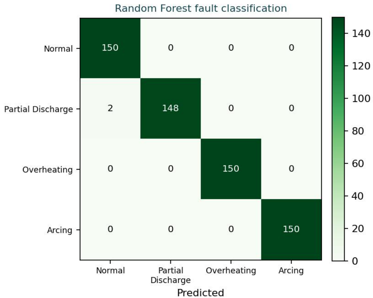
Fig. 4. Random Forest confusion matrix on held-out condition data (0.997 accuracy).
