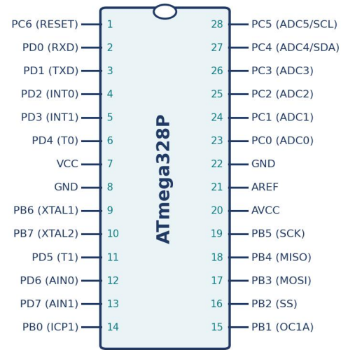
Fig. 2. ATmega328P microcontroller pin configuration.
