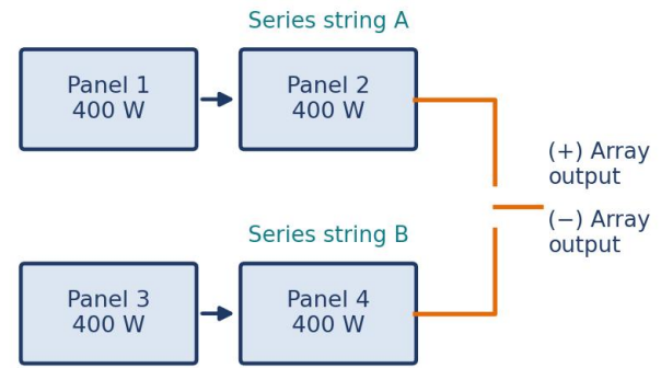
2S2P topology: two series strings connected in parallel
