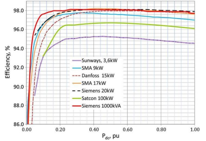
Fig. 1. Inverter efficiency metrics (adapted from [16], p. 5).
