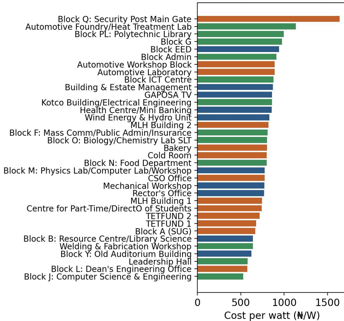
Figure 3. Buildings ranked by cost per watt, colour
