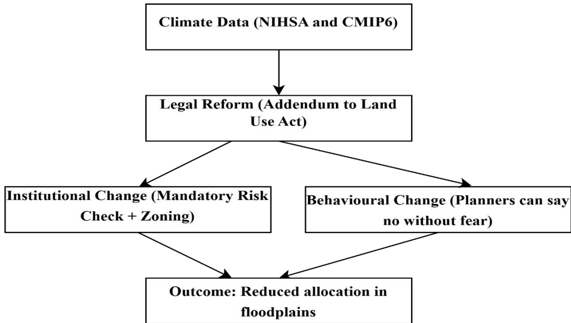
Fig 1: Conceptual Framework Linking Climate Data, Legal Reform, Institutional Change, and Behavioural Change to Reduced Floodplain Allocation.
