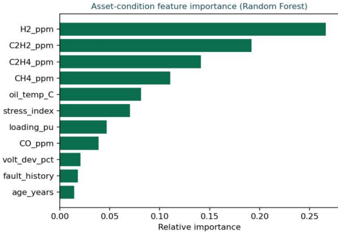
Fig. 2. Feature importance. Hydrogen, acetylene and ethylene carry the most diagnostic weight.
