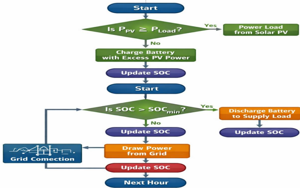
Figure 3. Hourly Energy Dispatch Algorithm for Hybrid PV–Battery System
