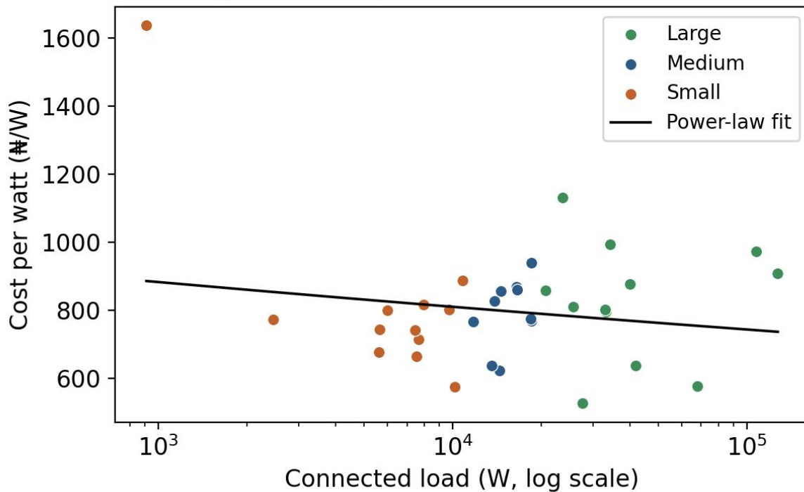
Figure 2. Cost per watt vs. connected load
