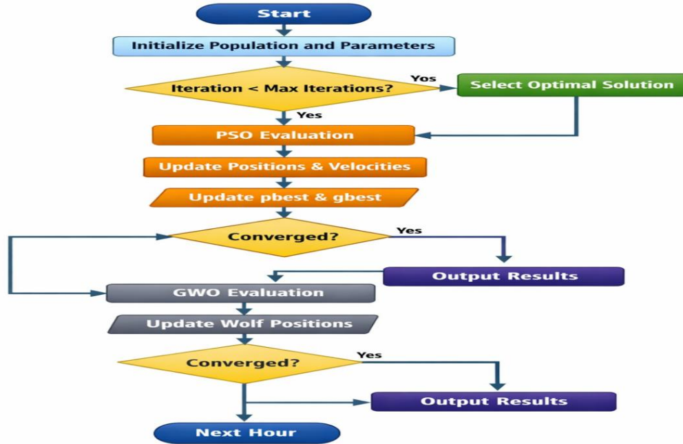
Figure 4. PSO and GWO Optimisation Procedure for Hybrid PV–Battery System
