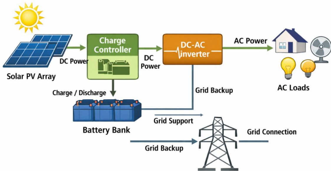
Figure 2. Block Diagram of Hybrid Solar PV–Battery System
