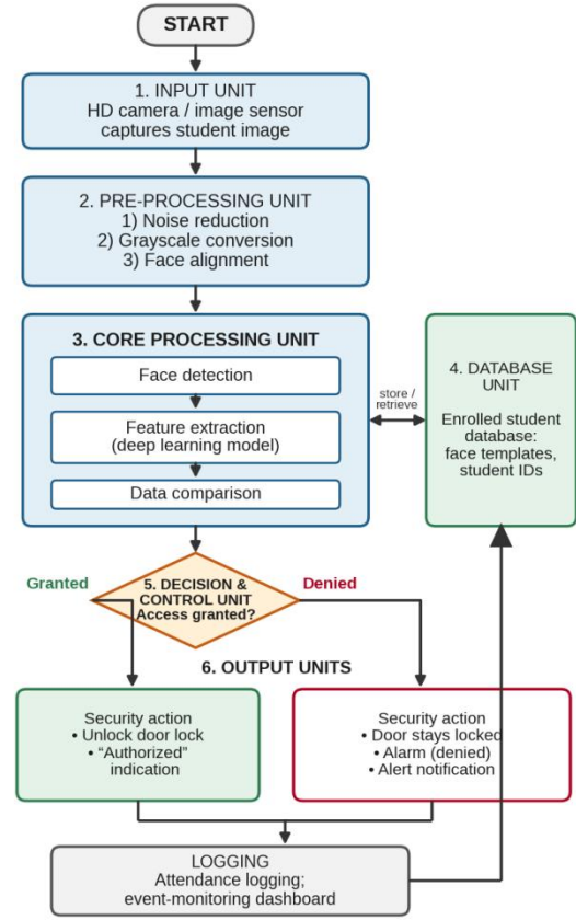
Fig. 1. Software/logic flowchart for the AI-based face recognition and access-control system.
