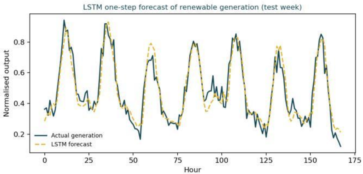
Fig. 3. LSTM one-step generation forecast against ground truth over a test week.
