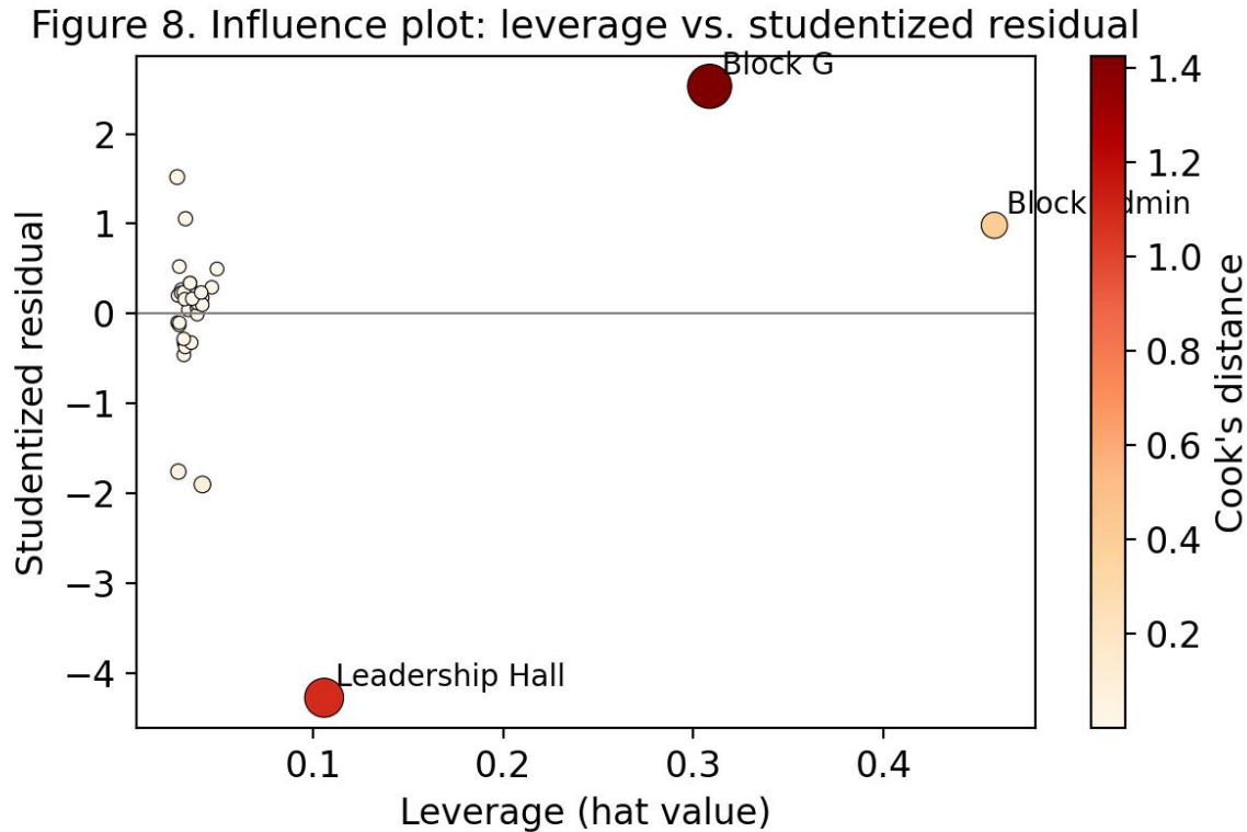
Fig. 8. Influence plot: leverage vs. studentized residual, with marker size and colour proportional to Cook's distance. The three most influential buildings (Block G, Leadership Hall, Block Admin) are individually labelled.
