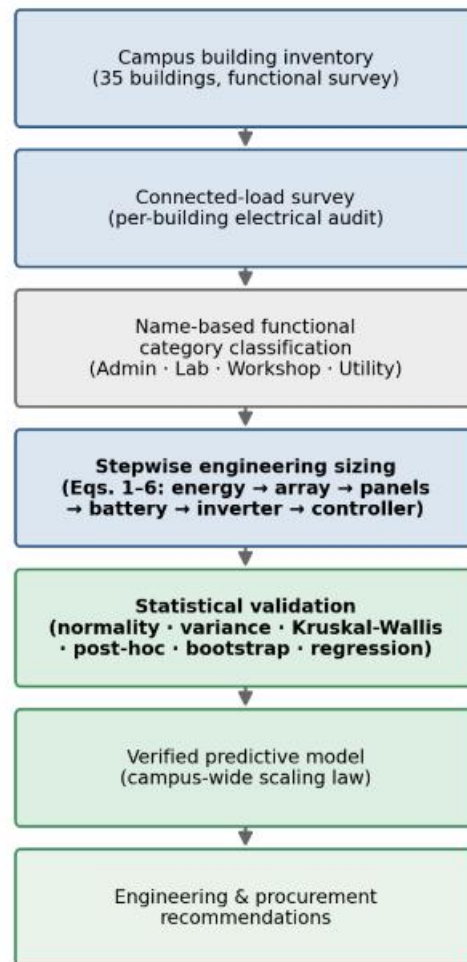
Fig. 1. Overall research and sizing methodology workflow, from campus building inventory through to engineering and procurement recommendations.
